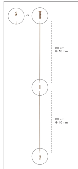
Suspension Kit
